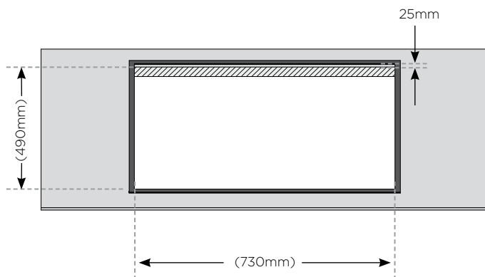
Figure 6b - Mastic seal position (WHG756SB)
