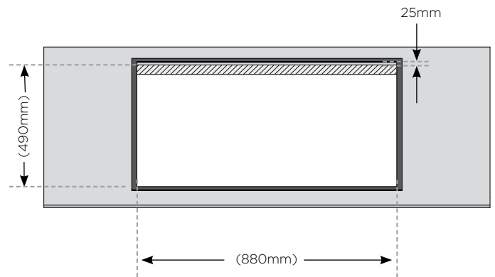
Figure 6c - Mastic seal position (WHG952SB & WHG956SB)
